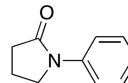
N-phenylazacyclopentan-2-one
