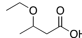
3-ethoxybutanoic acid
