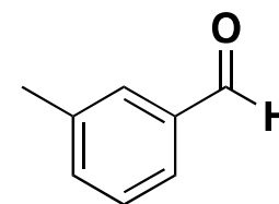
3-methylbenzaldehyde
