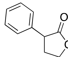
3-phenyloxacyclopentan-2-one
