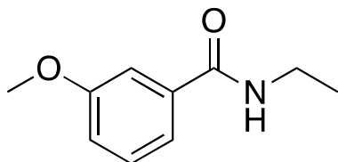
N-ethyl-3-methoxybenzamide
