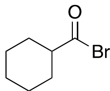
cyclohexanecarbonyl bromide
