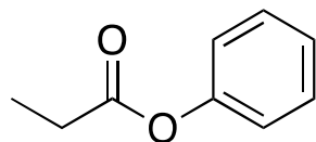
phenyl propanoate
