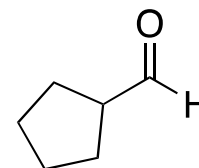
cyclopentanecarbaldehyde
