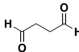
butanedial
