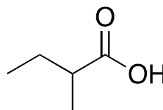
2-methylbutanoic acid
