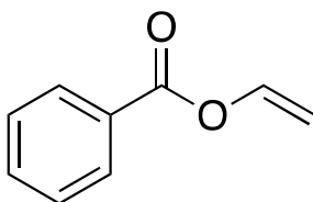
ethenyl phenylcarboxylate
