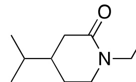
N-ethyl-4-(2-propyl)azacyclohexan-2-one
